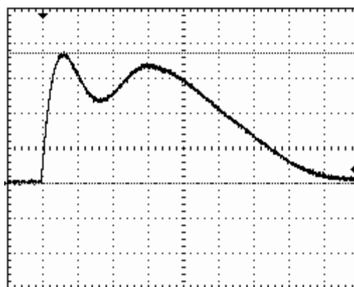
Fig. 15. Oscillogram of the aperiodic current pulse of 17/265 \mu\text{s} of artificial lightning in the high-current discharge circuit of the powerful high-voltage generator ГТМ-10/350 at EE of a solid round aluminum core with cross section of 6 \text{mm}^2 and length of 0,5 m of a network wire АППБНГ2×6 with polyvinyl chloride insulation ( U_{C1-3} \approx 15 \text{ kV} ; U_{C4} \approx 2.1 \text{ kV} ; I_m \approx 83.8 \text{ kV} ; J_a \approx 1.41 \cdot 10^6 \text{ J}/\Omega ; q_0 \approx 31.7 \text{ C} ; \tau \approx 17 \mu\text{s} ; \tau_p \approx 265 \mu\text{s} ; vertical scale – 22.52 kA/division; horizontal scale – 50 \mu\text{s} /division) [20]
