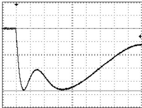
Fig. 12. Oscillogram of an aperiodic current pulse of the time shape of 15/340 \mu\text{s} in the high-current discharge circuit of the powerful high-voltage generator of artificial lightning current type ГТМ-10/350 with a low-resistance RL -load ( U_{C1-3} \approx 15 \text{ kV} ; U_{C4} \approx 2.25 \text{ kV} ; I_m \approx 106 \text{ kA} ; J_a \approx 3.03 \cdot 10^6 \text{ J}/\Omega ; q_0 \approx 52.2 \text{ C} ; \tau \approx 15 \mu\text{s} ; \tau_p \approx 340 \mu\text{s} ; R_H \approx 0.1 \Omega ; L_H \approx 1.5 \mu\text{H} ; vertical scale - 22.52 kA/division; horizontal scale - 50 \mu\text{s} /division) [19]
