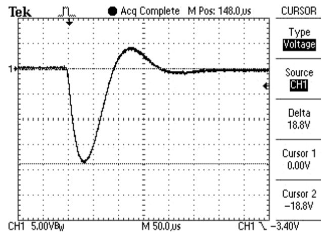
Fig. 3. Oscillogram of the pulsed A - component of the artificial lightning current with normalized ATPs in the high-current discharge circuit of the high-voltage generator PSG-A of the powerful domestic GCL of the YITOM-1 type ( U_{3A} \approx 29.7 kV; I_{mA} \approx -212 kA; J_{aA} \approx 2.09 \cdot 10^6 J/ \Omega ; \tau_f \approx 32 \mu s; \tau_p \approx 500 \mu s, vertical scale – 56.3 kA/division, horizontal scale – 50 \mu s/division)
