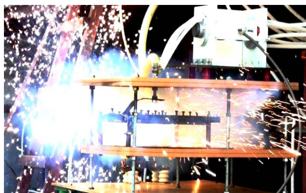
Fig. 14. General view of the EE phenomenon of a solid round aluminum core of 6 \text{mm}^2 cross-section of the АППБНГ2×6 network cable with polyvinyl chloride insulation in the high-current discharge circuit of the powerful high-voltage generator type ГТМ-10/350 ( U_{C1-3} \approx 15 \text{ kV} ; U_{C4} \approx 2.1 \text{ kV} ; I_m \approx 83.8 \text{ kV} ; J_a \approx 1.41 \cdot 10^6 \text{ J}/\Omega ; q_0 \approx 31.7 \text{ C} ; \tau \approx 17 \mu\text{s} ; \tau_p \approx 265 \mu\text{s} ) [20]
