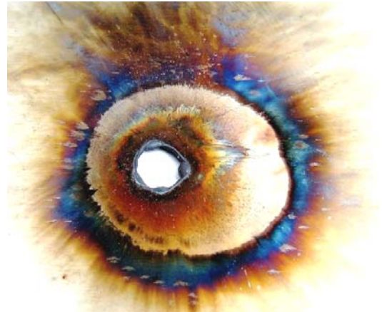
Fig. 7. General view of the affected area in an experimental sheet specimen made of stainless steel grade 12X18H10T of 1 mm thickness from the direct simultaneous action on it of a pulsed A -component ( I_{mA} \sim 192 kA; J_{aA} \sim 1.9 \cdot 10^6 J/Ω; \tau_f \sim 34 μs; \tau_p \sim 500 μs) and a long-term C - component of the artificial lightning current ( I_{mC} \sim 804 A; q_{0C} \sim 165 C; \tau_f \sim 9 ms; \tau_p \sim 448 ms) formed in high-current discharge circuits of the powerful high-voltage GCL of the УИТОМ-1 type [16]
