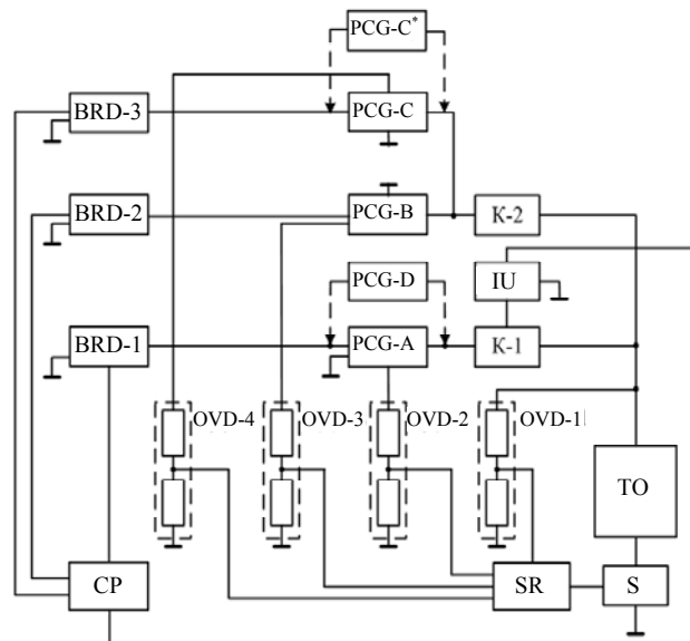
Fig. 2. Principal block electrical circuit for constructing a powerful lightning current generator of the type YITOM-1, containing individual pulse current generators PSG-A, PSG-B, PSG-D, PSG-C and PSG-C* (K-1, K-2 – high-voltage air switches for \pm 50 and \pm 5 kV; IU – ignition unit for \pm 100 kV; BRD-1, BRD-2 and BRD-3 – boost-rectifying devices for charging high-voltage capacitors of generators PSG-A, PSG-B, PSG-D, PSG-C and PSG-C*, CP – control panel, OVD-1, OVD-2, OVD-3 and OVD-4 – ohmic voltage dividers for voltage measurement on capacitors of generators PSG-A, PSG-B, PSG-D, PSG-C and PSG-C*, SR – system for recording measured voltages and currents in the circuits of generators PSG-A, PSG-B, PSG-D, PSG-C and PSG-C*; S – measuring shunt; TO – tested object) [11]
