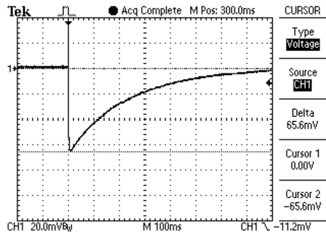
Fig. 4. Oscillogram of the long-term C - component of the artificial lightning current with normalized ATPs in the high-current discharge circuit of the high-voltage generator PCG-C* of the powerful GCL of the YITOM-1 type ( U_{3C} \approx -4 kV; I_{mC} \approx -738 A; q_{0C} \approx -182 C; \tau_f \approx 9 ms; \tau_p \approx 1000 ms, vertical scale – 225 A/division, horizontal scale – 100 ms/division)
