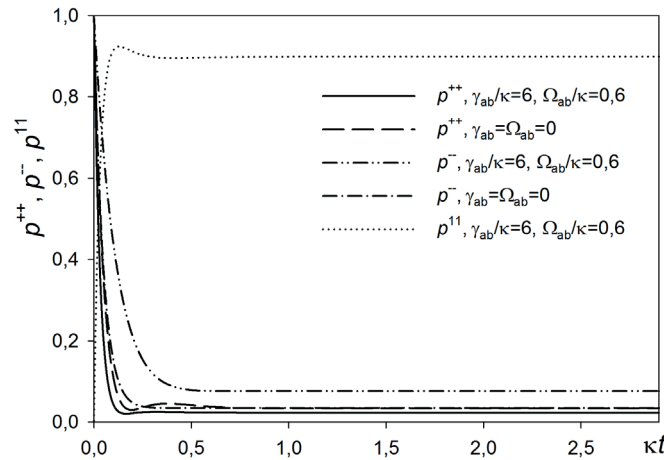
Fig. 3. Time evolution of different atomic states (with and without dipole-dipole interaction); p^{11}(t) = \text{Sp}_f[\rho_{nn}^{\alpha_1 \alpha_1}] is the probability of finding an atomic subsystem in state |\alpha_1\rangle . System parameters and notations are the same as in Figs. 1 and 2.
