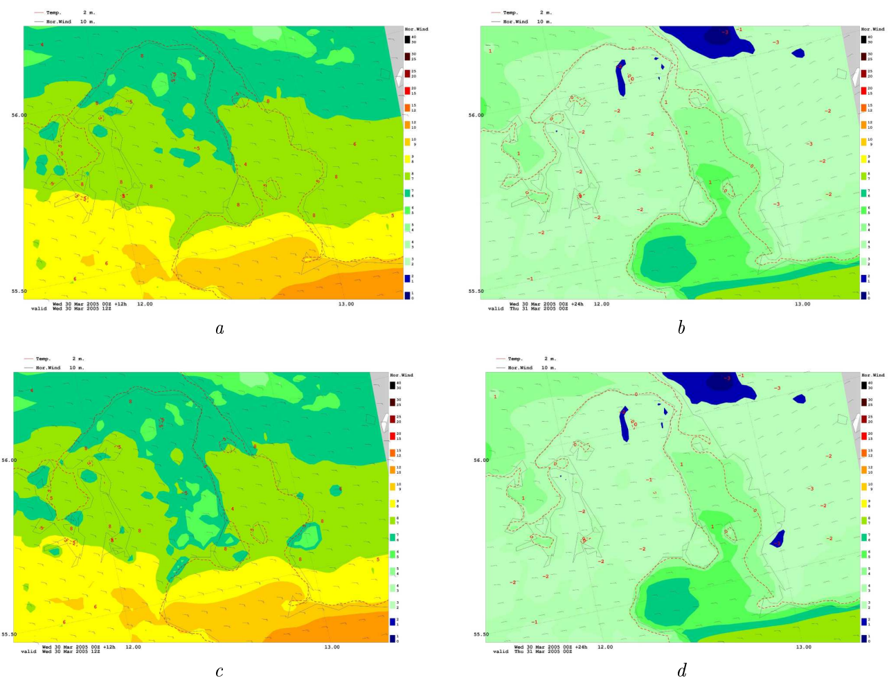
Fig. 2. DMI-HIRLAM simulated wind at 10 m and temperature at 2 m fields for roughness of 0.05 m ( a , b ) vs. modified roughness of 1 m ( c , d ) for 12 ( a , c ) and 24 ( b , d ) hour forecasts on 30 March 2005.
