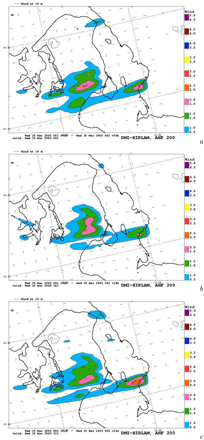
Fig. 3. Difference plots (between outputs of the DMI-HIRLAM control vs. modified run with addition of anthropogenic heat flux up to 200 \text{ W/m}^2 ) for wind velocity at 10 m at: a — 06, b — 18, and c — 24 UTC forecasts on 30 March 2005.
