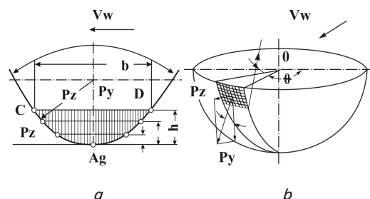
Fig. 8. Schemes of rounded edges of cutting grains [30]: a – the projection of the section of the rounded cutting edge of the grain on the plane, b – the view in the axonometry of the rounded cutting edge of the grain
