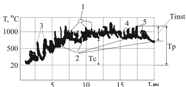
Fig. 1. Characteristic shape of the heat pulse during grinding: 1, 3, 4, 5 — temperature flares from the cutting grains, T_c — contact temperature, T_i — instantaneous temperature of grain cutting, T_p — pulse temperature — the sum of contact and instantaneous
