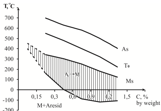
Fig. 7. Assumed position of the lines T_0 (equilibrium temperature) and A_s (austenite formation start temperature)
