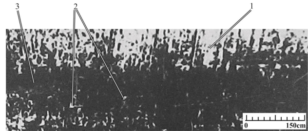
Fig. 4. Microsection of type “oblique cut” 5°. 1 – the end of the ground surface, 2 – small austenite spots, 3 – tempered layer. \times 150
