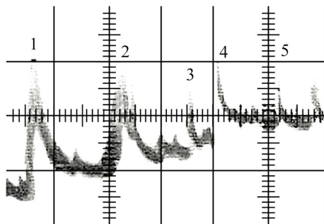
Fig. 3. Cut-out from the heat pulse of contact temperature
