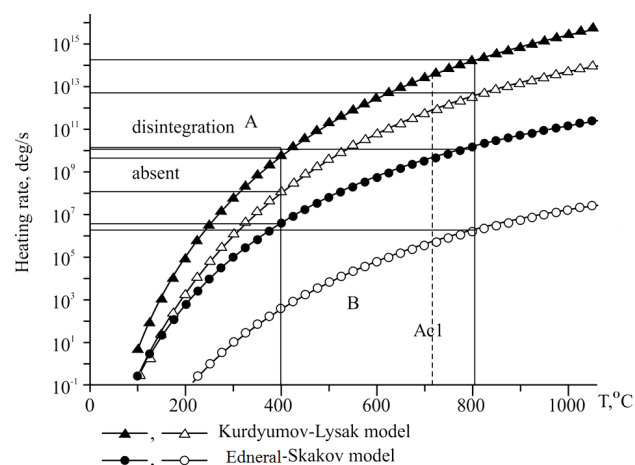
Fig. 2. Areas of possible diffusion decay of martensite as a function of the heating rate
