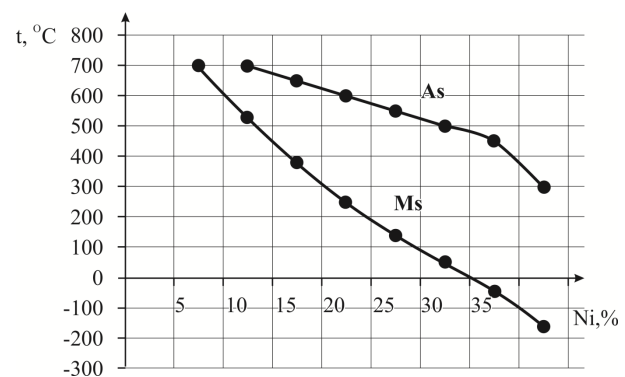
Fig. 6. Temperatures of the start of direct M_s and reverse A_s martensitic transformation [23]
