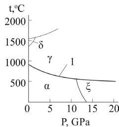
Fig. 9. Equilibrium line \alpha \rightarrow \gamma for iron, depending on temperature and pressure [24, 30]
