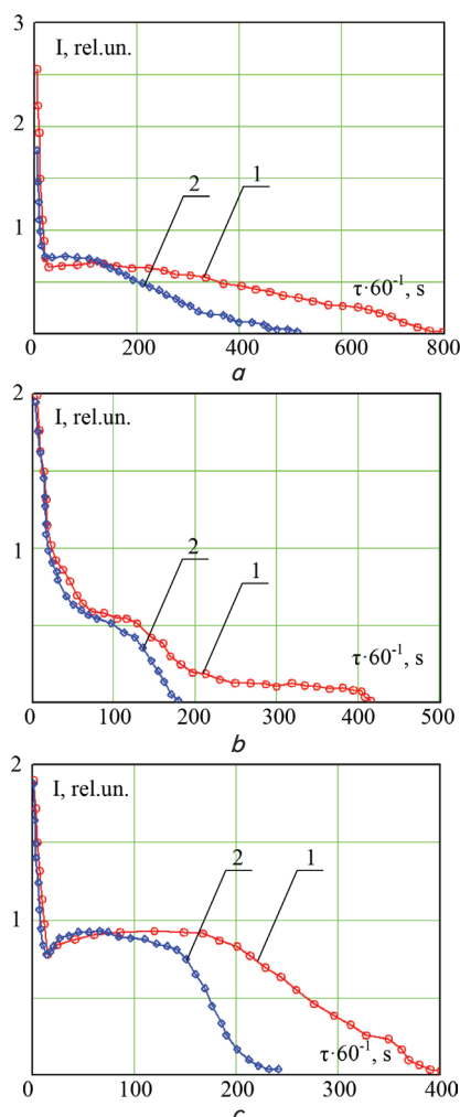
Fig. 5. Thermograms obtained by the calorimetric method at calorimeter temperature of -12\text{ }^{\circ}\text{C} for model food systems: No. 1 (yeast dough) (a); No. 2 (puff pastry dough) (b); No. 3 (unleavened dough) (c)
