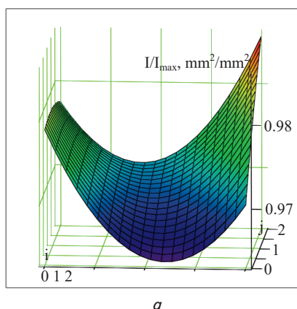
Fig. 2. Results of EPR studies: areas under the spectrum at different coordinates of the sample of the model food system No. 1 (yeast dough) ( a ); the surface tomogram ( b )
