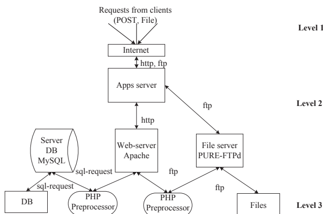
Fig. 6. Multilevel model of software organization of the server part of the system
