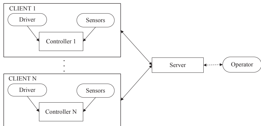
Fig. 1. Structure of the system for passenger traffic registration in the “smart” city
