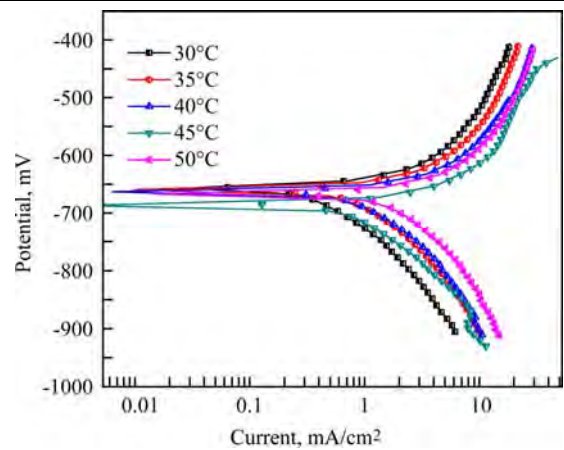
Fig. 5. Potentiodynamic polarization plots for the corrosion of 6061 Al-15 vol. pct. of SiC (p) composite in 0.25M HCl at different temperatures.
