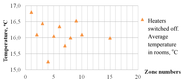
Fig. 4. Results of the temperatures study in the working zones of non-heated rooms
