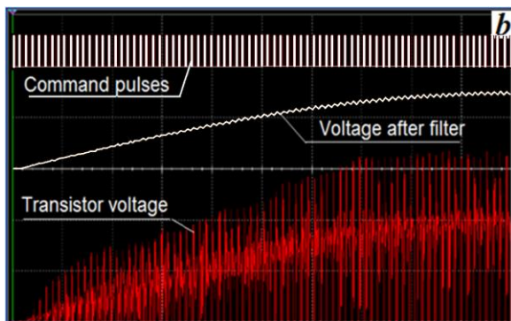
Fig. 9. Voltage curve on the filter capacity C1 = 2500 \text{ nF} .
