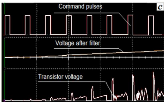
Fig. 7. Control pulse diagrams, transistor voltages and voltage curve on after rectifier (shown in different scale sizes to elucidate the process, scale a < \text{scale } b < \text{scale } c ).
