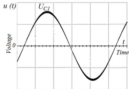
Fig. 9. Voltage curve on the filter capacity C1 = 2500 \text{ nF} .
