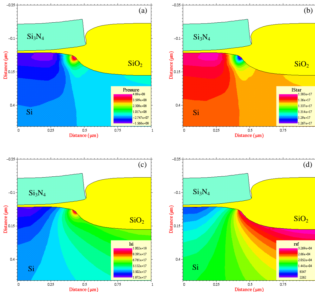
Figure 2: Contour plots of simulated (a) pressure (Pa), (b) equilibrium concentration and (c) concentration of interstitials ( \text{cm}^{-3} ), (d) stacking fault radius ( \text{\AA} ) after steam field oxidation performed at 1100\text{ }^{\circ}\text{C} . Stress-dependent surface generation and recombination of point defects was taken into account.
