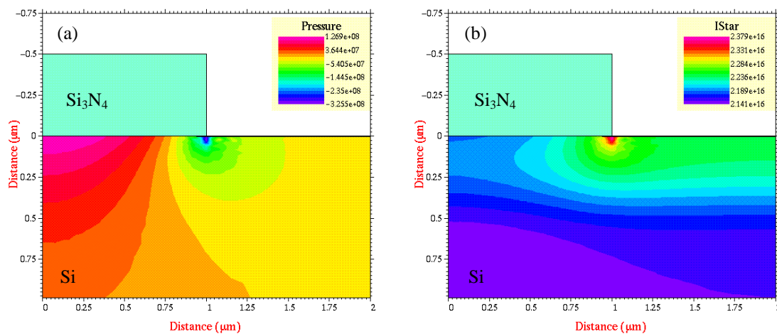
Figure 3: Simulated (a) pressure (Pa) and (b) equilibrium concentration of interstitials ( \text{cm}^{-3} ) after 1014 °C anneal in \text{N}_2 for 120 min.
