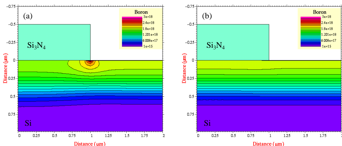
Figure 6: Contour plots of simulated boron concentration ( \text{cm}^{-3} ) after 1014^\circ\text{C} anneal in \text{N}_2 for 120 min (a) with and (b) without accounting for stress-dependent surface generation and recombination of point defects.
