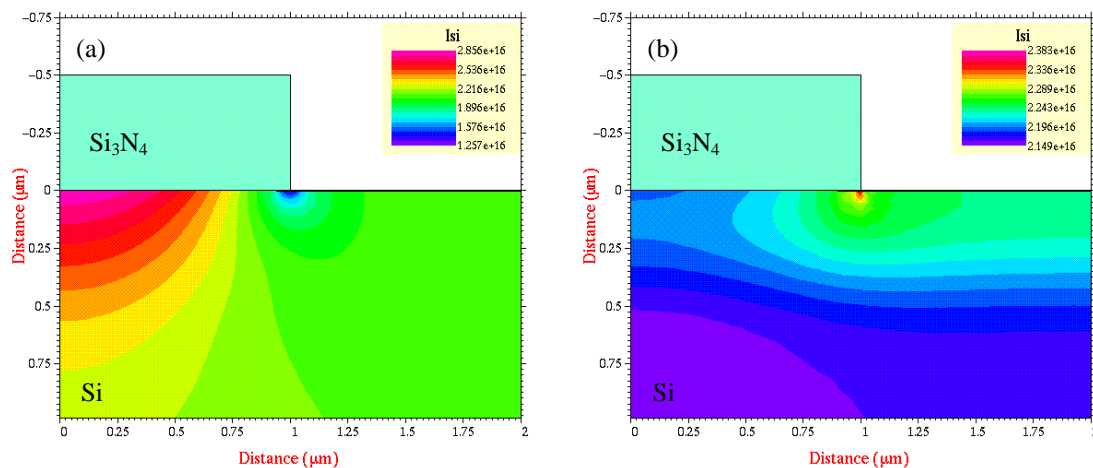
Figure 4: Simulated interstitial concentration ( \text{cm}^{-3} ) after 1014 °C anneal in \text{N}_2 for 120 min (a) with and (b) without taking into account stress-dependent surface generation and recombination of point defects.
