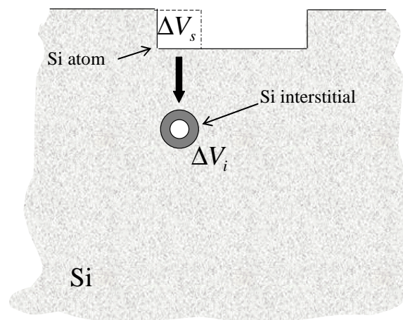
Figure 1: Self-interstitial formation in silicon by surface generation. \Delta V_s > \Delta V_i .
