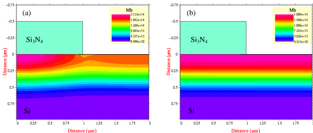
Figure 5: Simulated concentration of boron-interstitial pairs ( \text{cm}^{-3} ) after 1014^\circ\text{C} anneal in \text{N}_2 for 120 min (a) with and (b) without accounting for stress-dependent surface generation and recombination of point defects.
